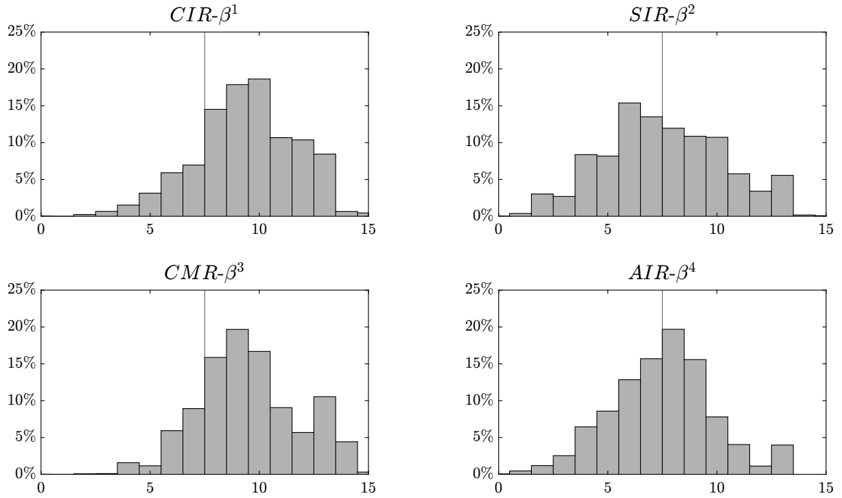
Figure B.8: Histogram of Overlapping Weights in Carry and Liquidity Risk Factors
