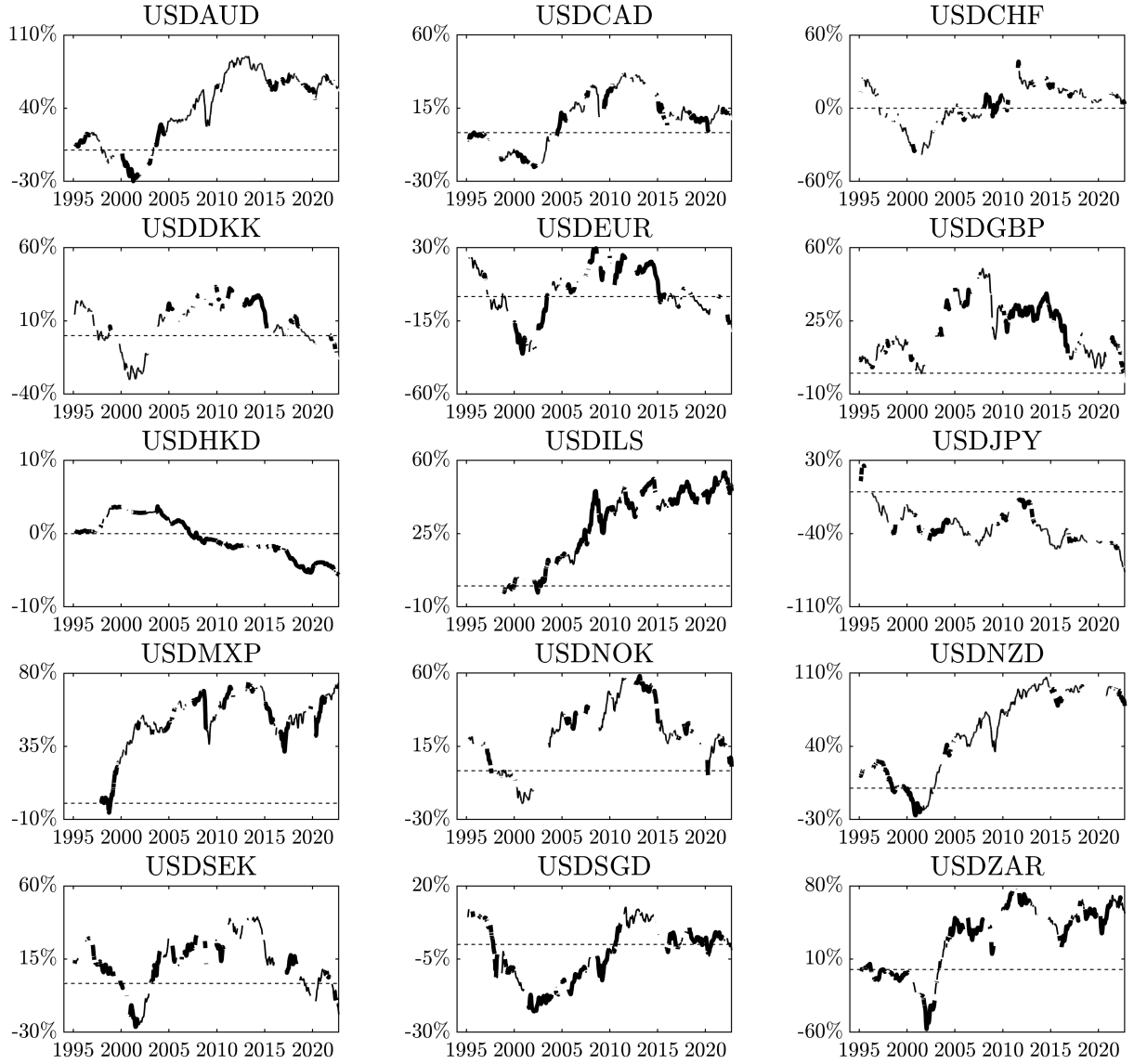
Figure B.6: Cumulative Excess Returns by Currency Pair ( CMR-\beta^3 )
