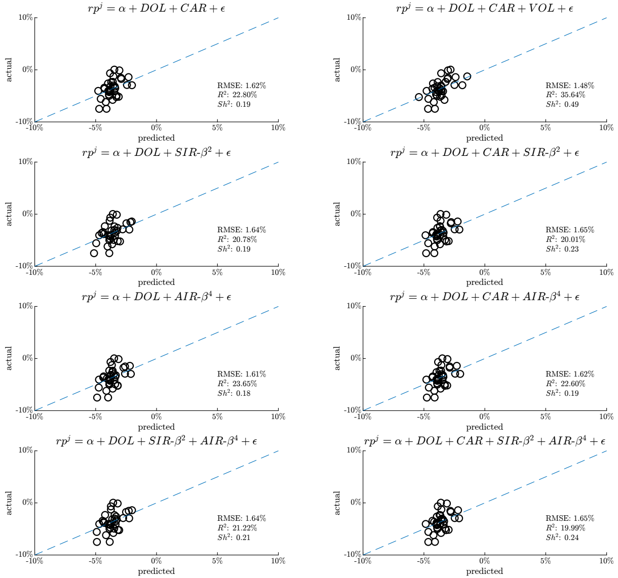
Figure B.10: Realised Versus Predicted Excess Return Conditional on Market Stress
