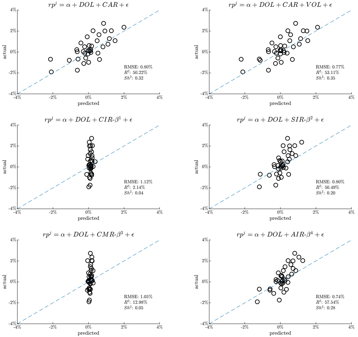
Figure B.15: Realised Versus Predicted Excess Return (UMVE)
