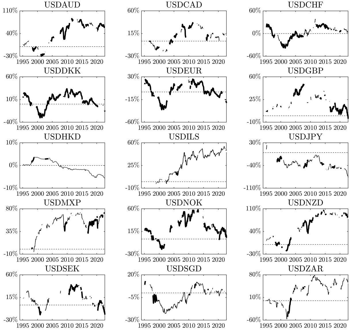
Figure B.4: Cumulative Excess Returns by Currency Pair ( CIR-\beta^1 )
