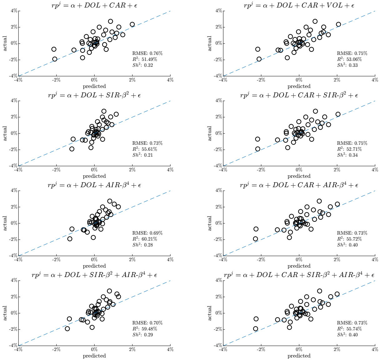
Figure 1: Realised Versus Predicted Excess Return
