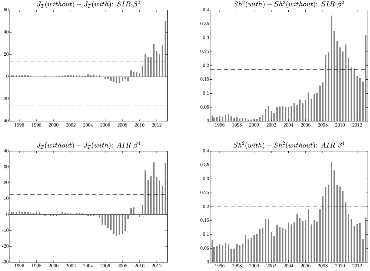
Figure 2: Liquidity Risk Factors and the Currency Pricing Kernel
