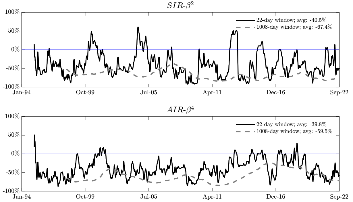
Figure 3: Cross-sectional Correlation of Moving Average Weights
