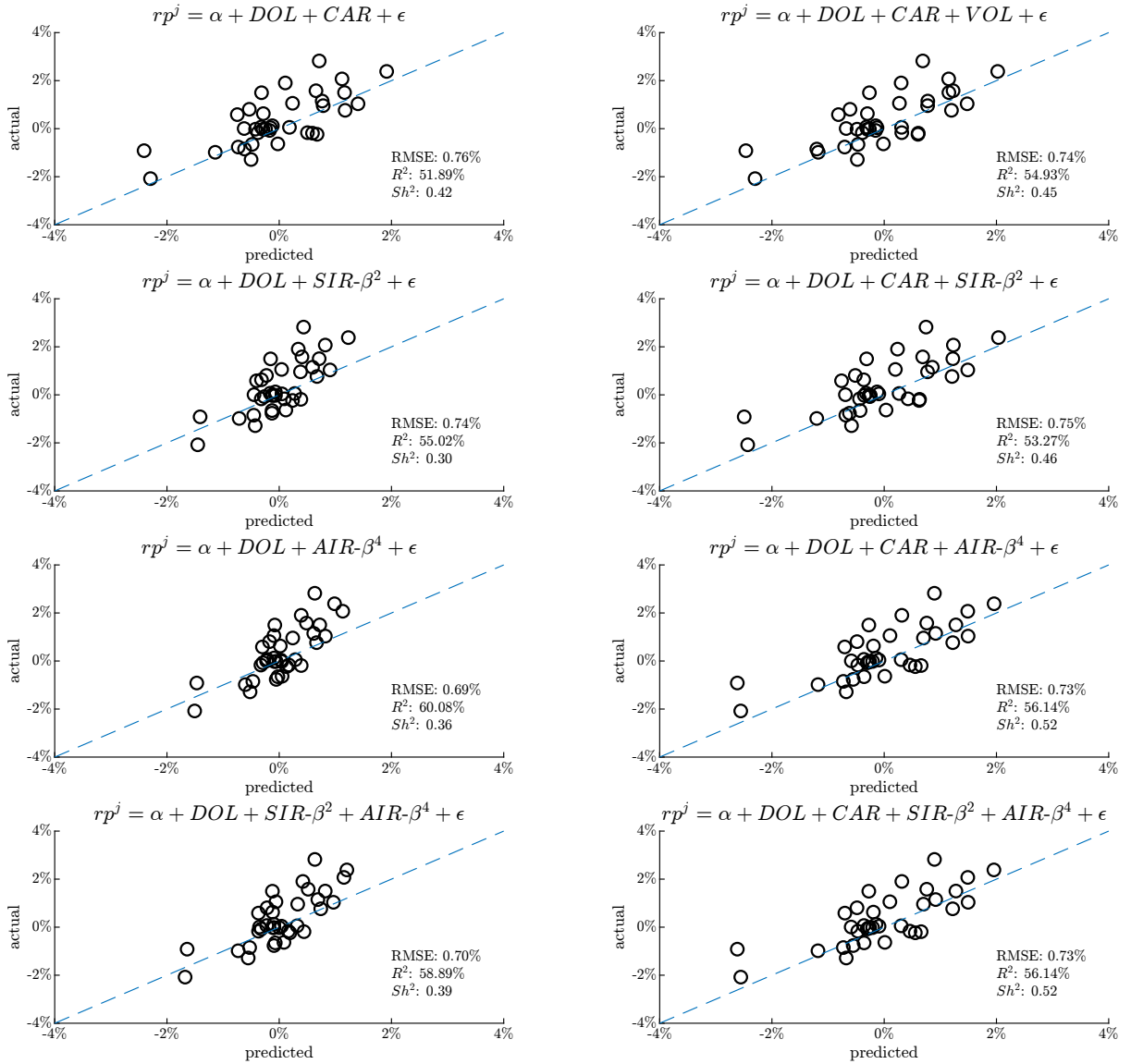
Figure B.12: Realised Versus Predicted Excess Return (Monthly)
