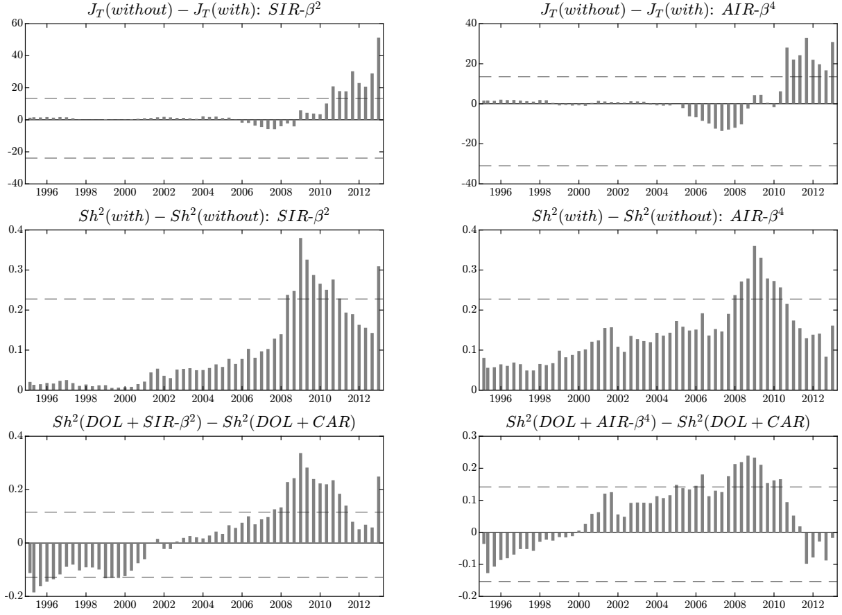
Figure B.11: Liquidity Risk Factors and the Currency Pricing Kernel
