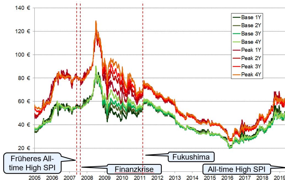
Figure 3: Development of futures prices on the EEX for 4 front years (Q1 05 - Q2 19).
