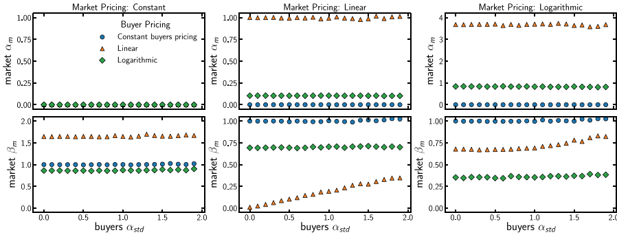
Figure 2. The Market's Parameters, as Regressed as a Function of the Standard Deviation of the Buyers, With Market Parameters \alpha_m (Upper Row) and \beta_m (Lower Row) as Regressed as a Function of the \alpha_{b,std} of the Buyers, Where Different Curves Represent Different Pricing Functions by the Buyers, and Different Columns Depict the Results for Constant, Linear, and Logarithmic Market Pricing (from l to r)
