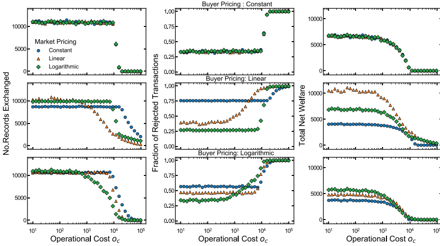
Figure 3. Global Properties of the Market as a Function of the Operational Cost, cost_c , Where the Upper, Middle, and Lower Panels Show the Results, Respectively, for Constant, Linear, and Logarithmic Pricing Functions, Followed by the Buyers, and the Left-Hand Panels Show the Number of Records Exchanged, the Middle Column the Number of Rejected Transactions, and the Right-Hand Column the Net Welfare, with Different Curves Representing Scenarios where The Market Implements Constant, Linear, or Logarithmic Pricing Functions as a Function of the Number of Requested Records
