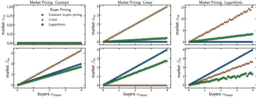
Figure 1. The Market's Parameters, as Regressed as a Function of the Mean of the Buyers, With Market Parameters \alpha_m (Upper Row) and \beta_m (Lower Row) as Regressed as a Function of the Mean \alpha_{b,mean} of the Buyers, Where Different Curves Represent Different Pricing Functions by the Buyers, While Different Columns Depict Results for Constant, Linear, and Logarithmic Market Pricing (from l to r)
