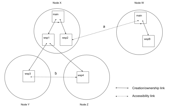
Figure 3: Distributed environment overview.
