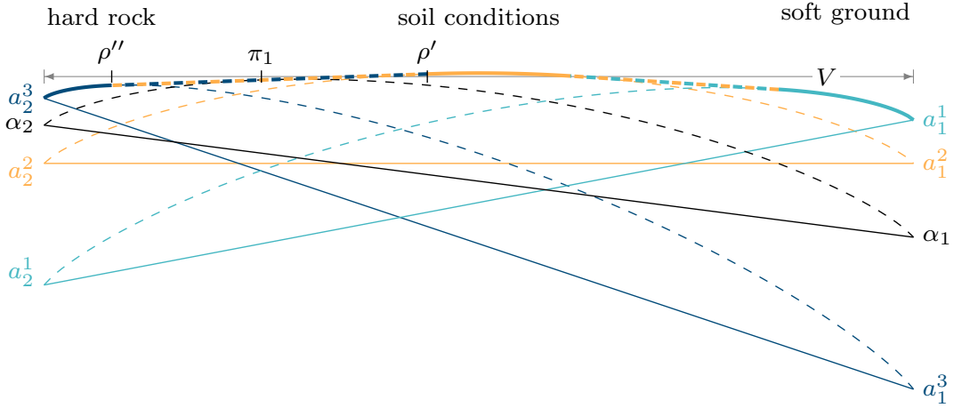
Figure 3: The introductory tunnel building example through the posterior-based lens. Monochrome dashed lines represent the net payoff for each action \mathbf{a} .
