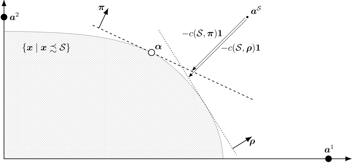
Figure 2: Dominated payoff vectors and construction of the ignorance equivalent.
