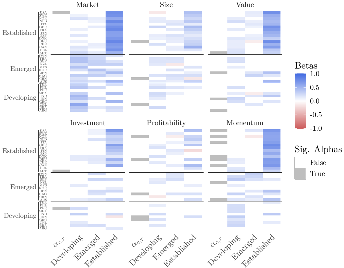
Figure 7: Spanning regressions of regional factor returns
