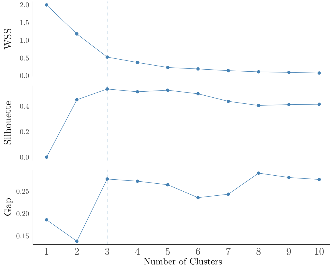
Figure A.6: Cluster statistics using the PAM algorithm
