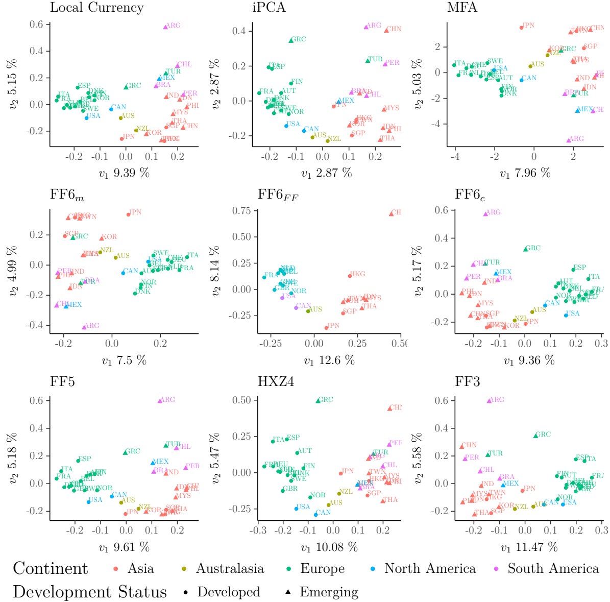
Figure A.7: Robustness of integrated principal component analysis of global factor returns. The plot illustrates the first two eigenvectors, v_1 and v_2 , and the percentage of explained variance of their respective eigenvalues for international factor returns of the Fama and French (2018) six-factor model returns in USD that were decomposed using the cPCA algorithm by Tang and Allen (2021). Each plot illustrates a modified version of this baseline setting where one of the methodological decisions was changed. "Local Currency" shows the results if returns are in domestic currency instead of the USD. "iPCA" and "MFA" displays the results of when the general iPCA or MFA algorithm was employed instead of the cPCA algorithm respectively. The remaining plots display the results for different factor models. "FF6 m " displays the results for the Fama and French (2018) six-factor model from which the market factor was removed. "FF6 FF " displays results for the Fama and French (2018) six-factor model that was created using the traditional factor formation methodology by Fama and French (2017). "FF6 c " displays the results for the Fama and French (2018) six-factor model where the profitability factor was calculated using cash profitability. "FF5" shows the results for the Fama and French (2015) five-factor model, "HXZ4" displays the results for the Hou et al. (2015) q-factor model, and "FF3" displays the results for the Fama and French (1993) three-factor model.
