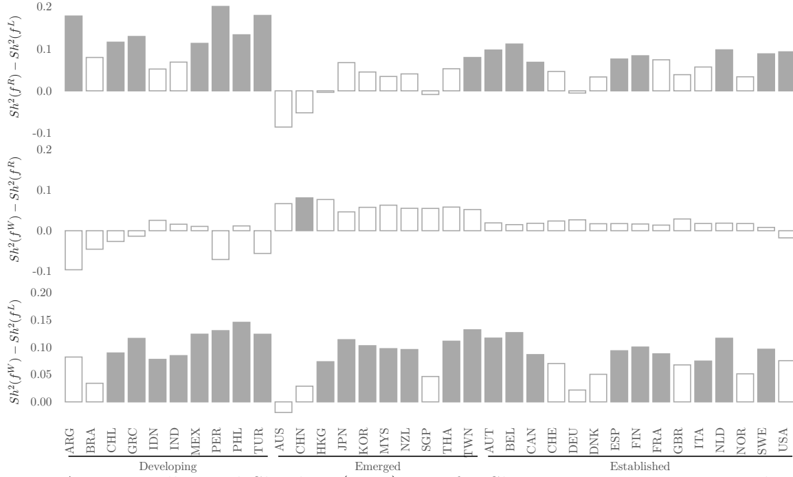
Figure A.10: Barillas and Shanken (2017) test for Sharpe ratio comparison with sorting aggregation procedure
