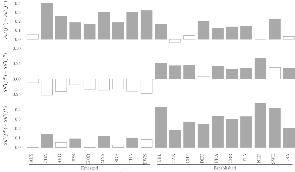
Figure A.9: Barillas and Shanken (2017) test for Sharpe ratio comparison with traditional Fama and French (2017) factor formation methodology
