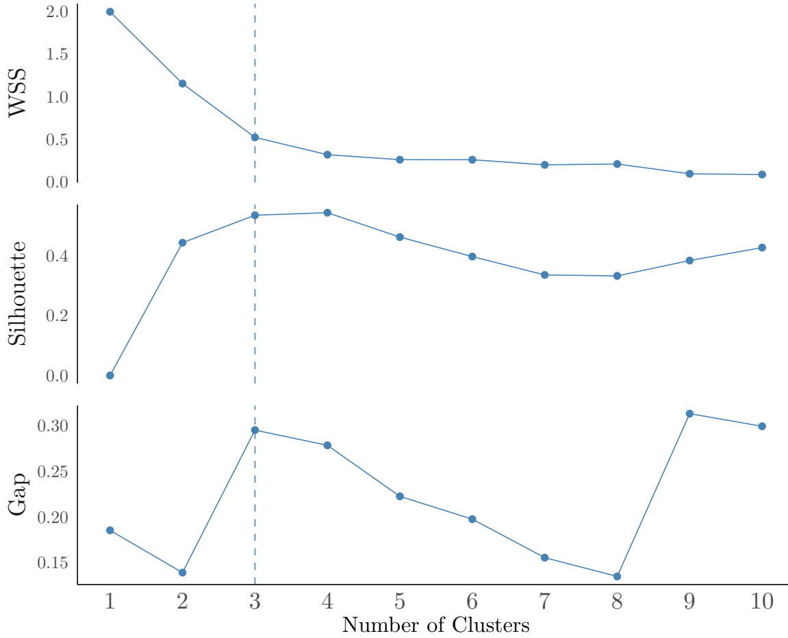
Figure A.5: Clustering statistics using the k-means algorithm
