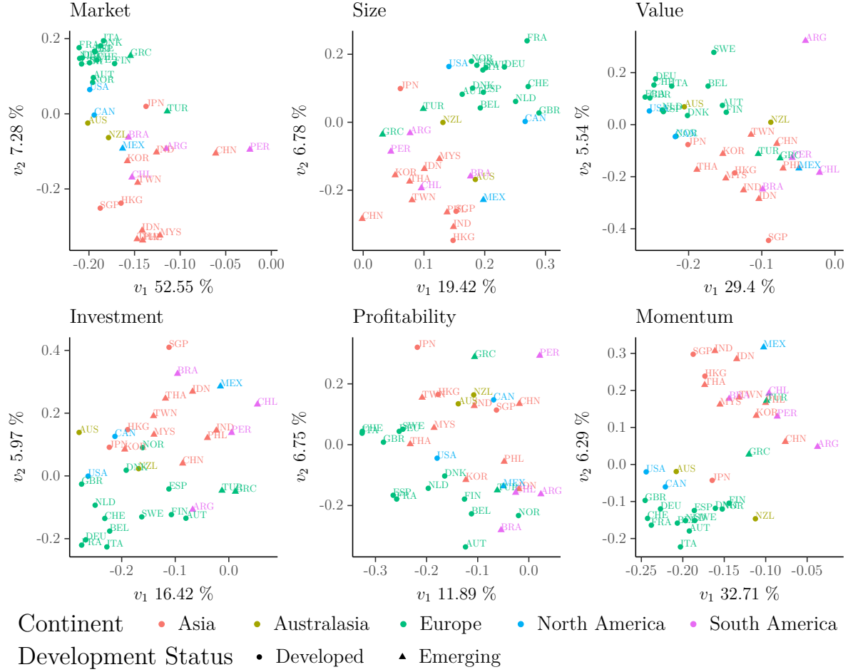
Figure 2: Principal component analysis of international factor returns
