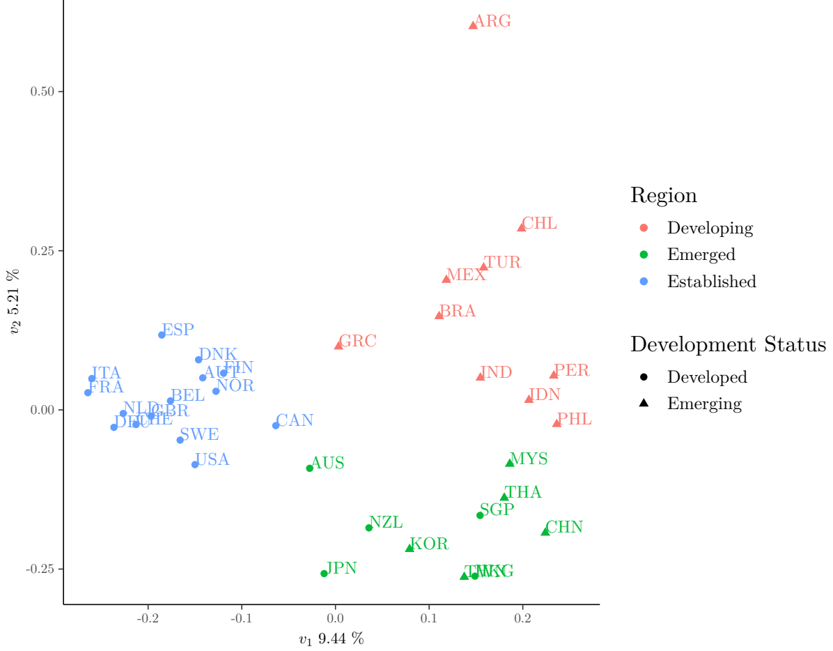
Figure 6: Principal component analysis of global factor returns with regions
