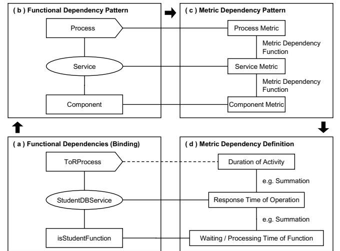
Fig. 1. Definition of Metric Dependencies
