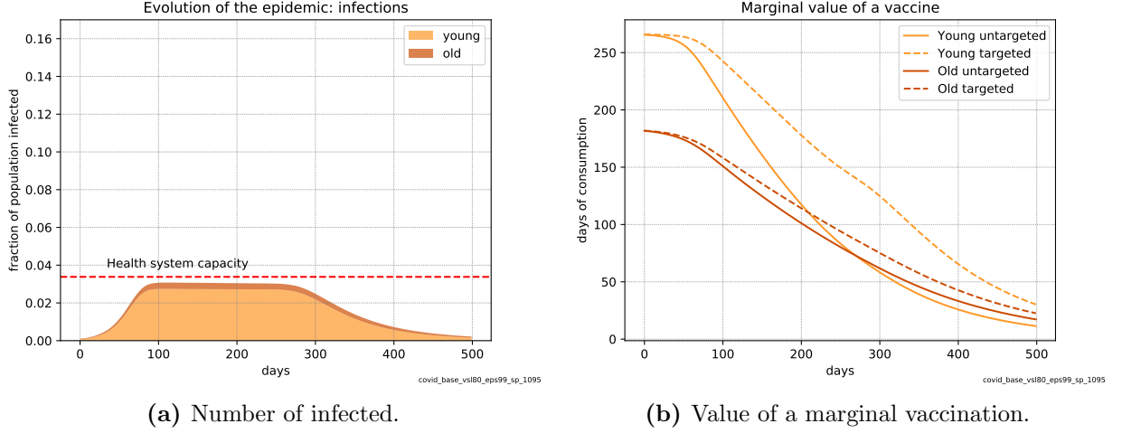
Figure 1: The marginal value of vaccination under the social-planner allocation.
