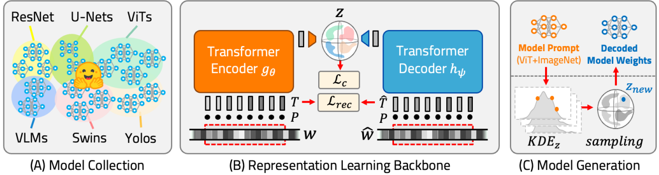
Figure 2. Overview of our approach. (A) A heterogeneous collection of models, including ViTs, Swins, ResNets, UNets, and vision-language models, is gathered from HuggingFace. (B) A weight-space autoencoder is trained to reconstruct and embed these models into a shared latent representation. (C) From this latent space, GeoSANE can generate new models on demand for specific downstream tasks such as flood segmentation, object detection, or land-cover classification.
