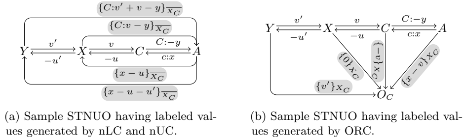
Fig. 3: Approach for managing values produced by two complementary rules.
