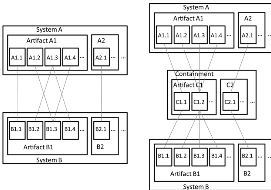
Fig. 1 Generic m:n mapping mechanism in systems theory
