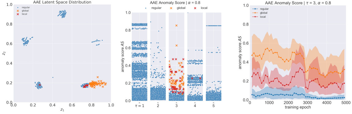
Figure 5: Learned AAE latent space representations of the journal entries contained in dataset A after training the AAE for 5,000 epochs and imposing a mixture of \tau = 5 Gaussians (left), the anomaly scores AS obtained for \alpha = 0.8 of each journal entry x_i and corresponding mode \mu_\tau (center), the anomaly score distribution (bold line defines the median, upper and lower bound define the 0.05 and 0.95 quantile of the distribution) obtained of each journal entry class with progressing network training (right).
