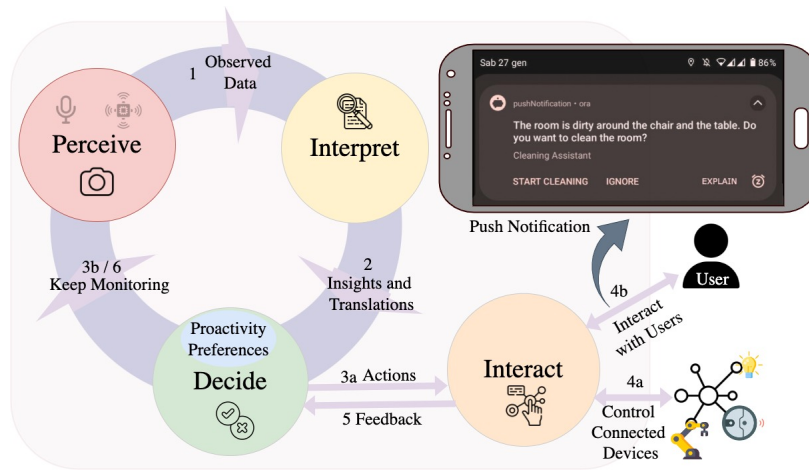
Figure 2: Phases of the system architecture of our proactive DC system. This augments the Decide phase of a personal DC [4] by adapting its proactivity level based on user preferences and interpretation of the context. In an example implementation scenario, the push notification suggests to start cleaning. The user may decline or accept the suggestion and also ask the DC to explain its actions.
