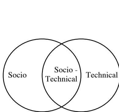
Fig. 3. Socio-Technical Model [3,8]
