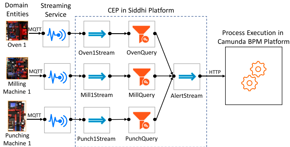
Fig. 11. Integration of IIoT event processing with the execution of a production process (Scenario 1).
