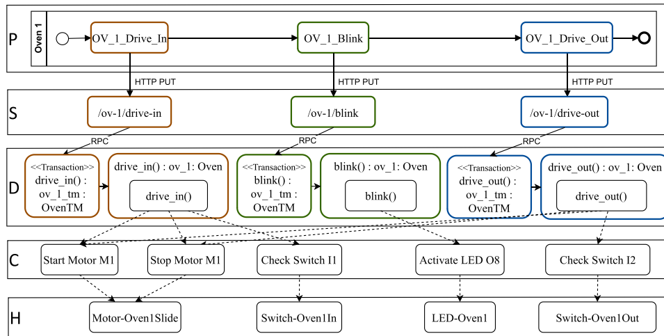
Fig. 9. Execution of Burn decomposed into three smaller process activities.
