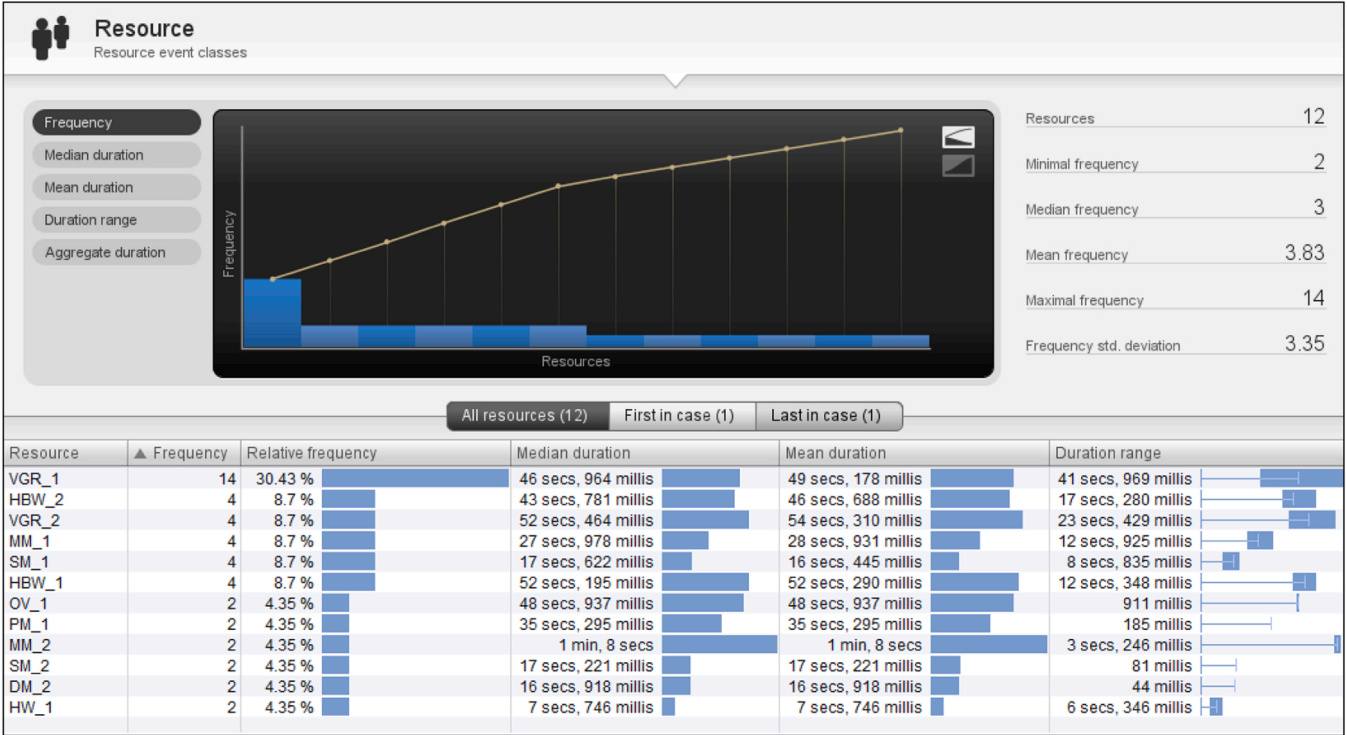
Fig. 14. Resource analysis obtained by a process mining tool.
