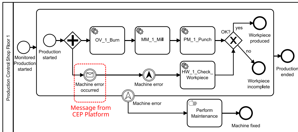
Fig. 10. Integration of a derived high-level process event in a production process (Scenario 1).
