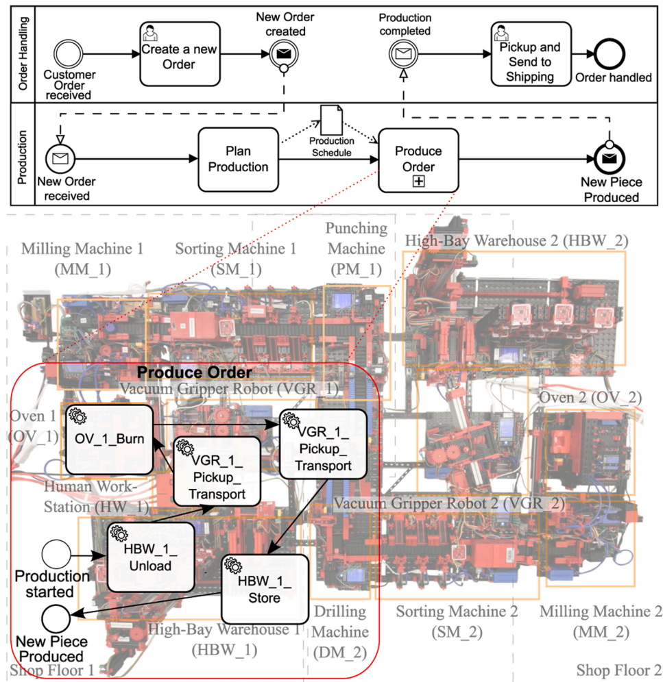
Fig. 7. Order-to-product process with production in our factory.
