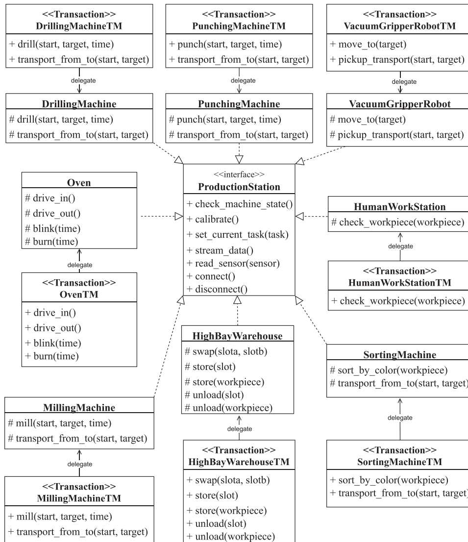
Fig. 4. Excerpt from the class diagram of the domain layer.
