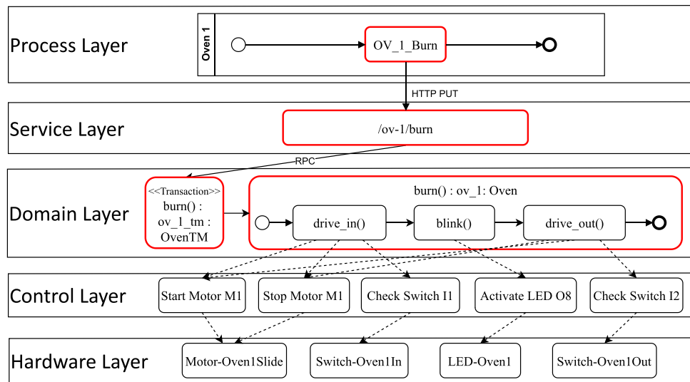
Fig. 8. Execution of Burn Encapsulated as one Atomic Process Activity.
