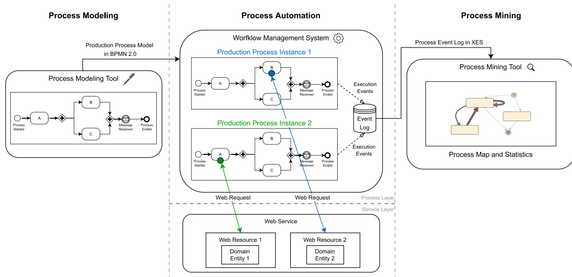
Fig. 5. Workflow among the BPM-related components on the process layer.
