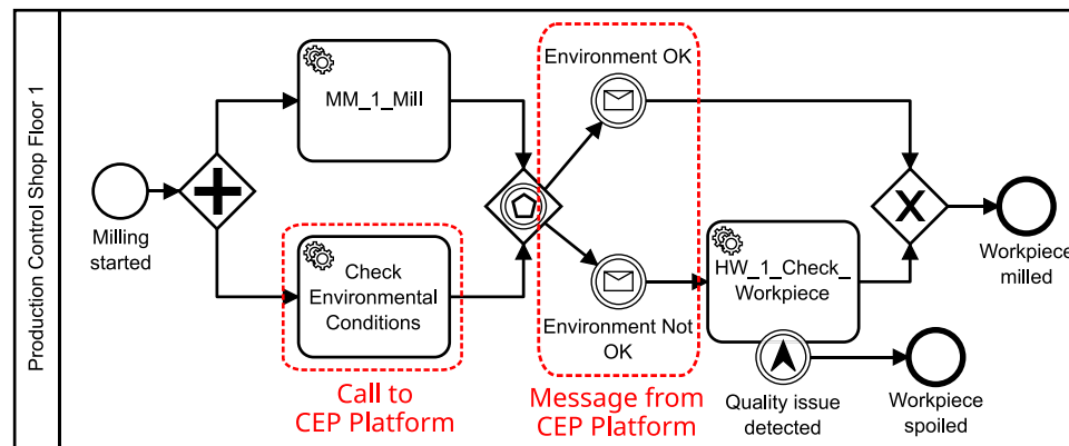
Fig. 12. Extension of a production activity with a check of environmental conditions (Scenario 2).
