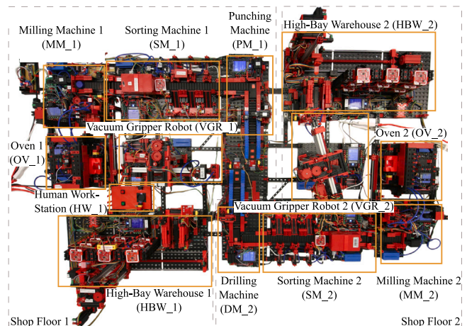
Fig. 3. Smart Factory Model used in this Work.
