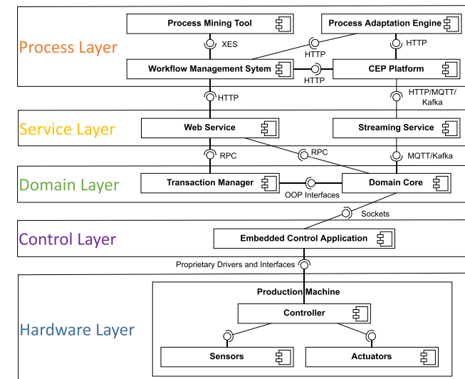
Fig. 2. Layers and components of the smart factory systems architecture.
