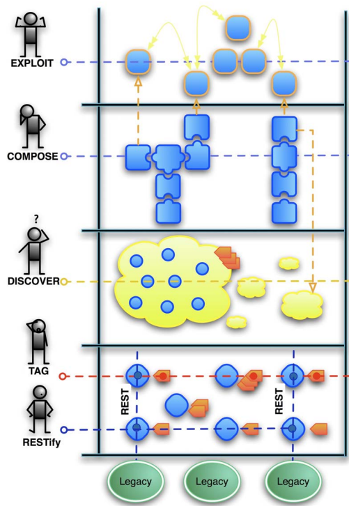
Figure 2. User-centered SOA solution stack
