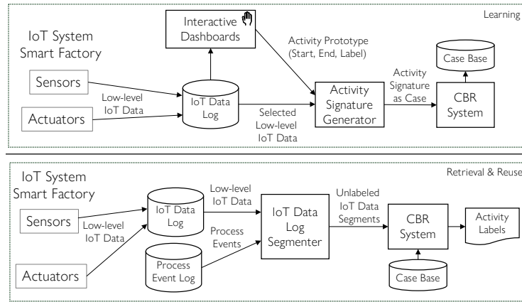
Fig. 3. Data flow Architecture for Learning and CBR Application.
