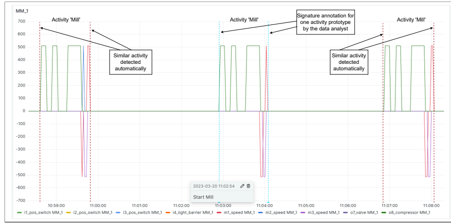
Fig. 2. IoT Data for three Instances of the Mill Activity with Signature Annotation for one Execution as Event Abstraction (middle, dashed light blue lines). The two similar instances (left and right, dashed dark red lines) should be detected automatically.
