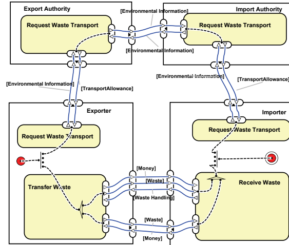
Fig. 2. Waste management example modeled with e3-Value notation
