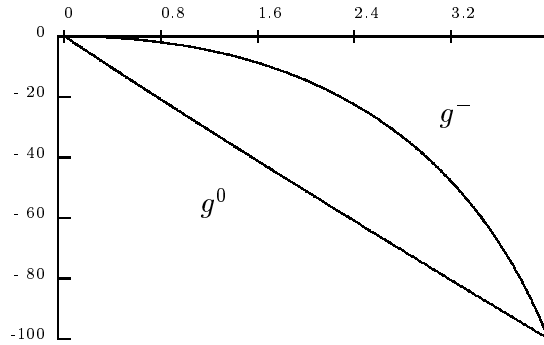
Figure 4: Risk profiles g^- and g^0
