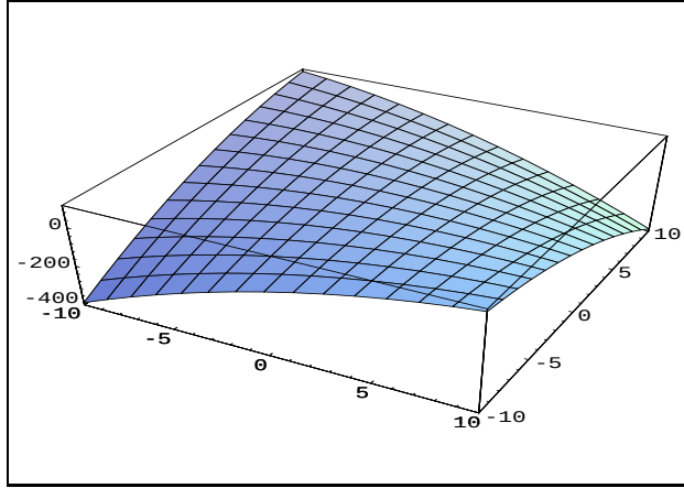
Figure 6: Hessian \Gamma = V^{-1}DV
