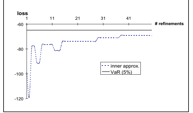
Figure 20: Convergence behavior in case b
