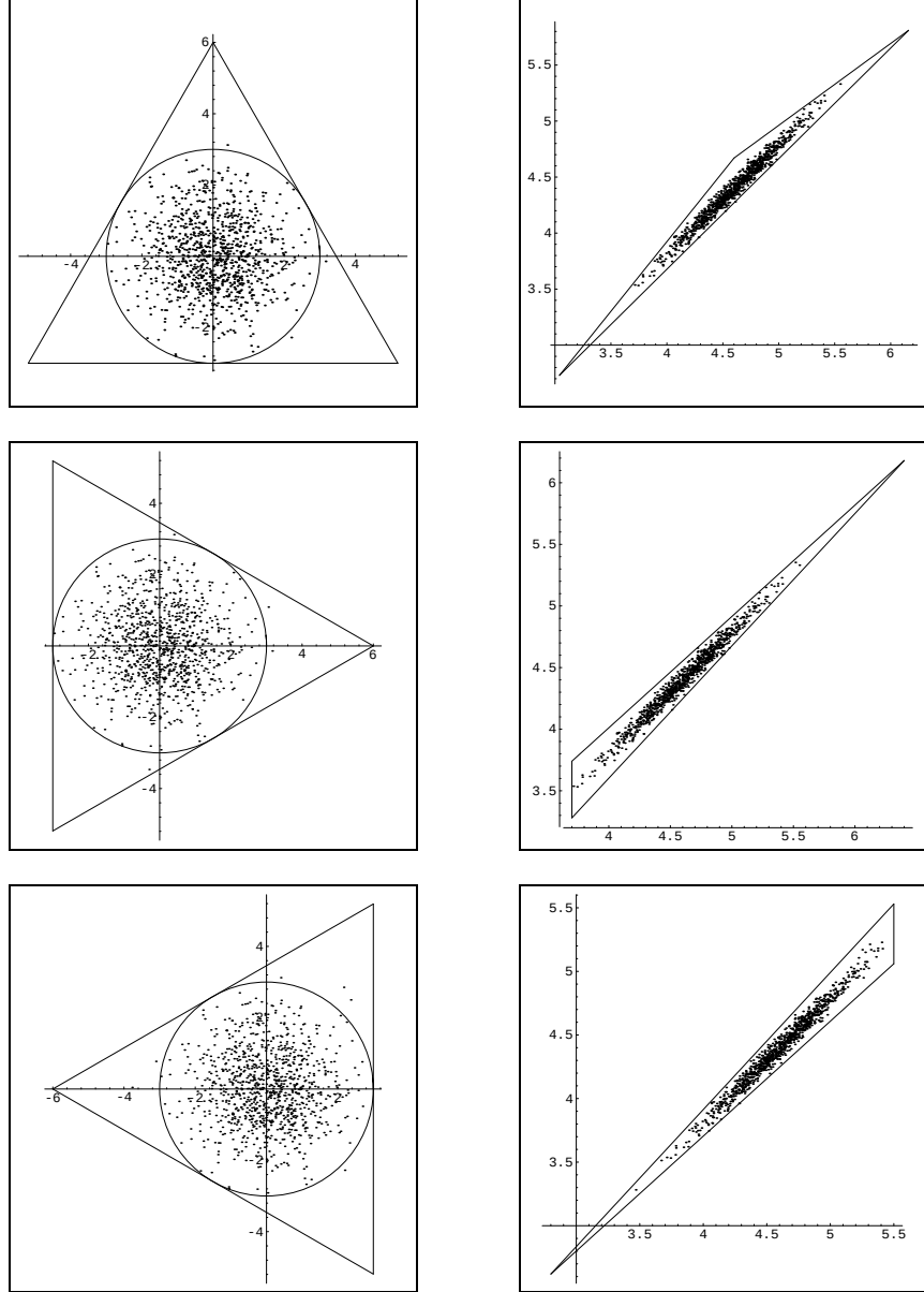
Figure 12: Various illustrations of a simplicial coverage
