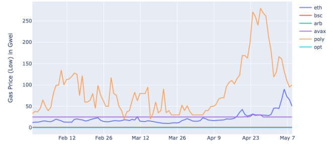
Fig. 2: Gas Prices [Gwei] over Time per Evaluation Chain
