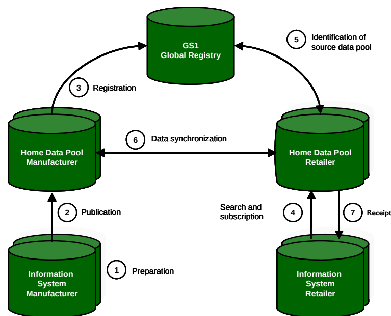
Figure 1: The Global Data Synchronization Network (GDSN)
